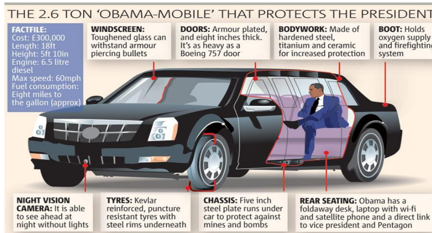
The USA Presidential “Beast” armored car
